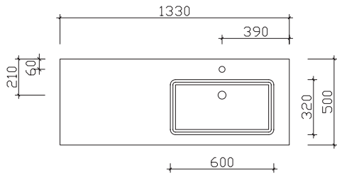
Width 1330 mm BRE015F13302
