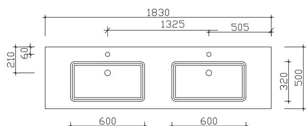
Width 1830 mm BMD015F18302
