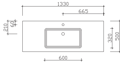
Width 1330 mm BME015F13302
