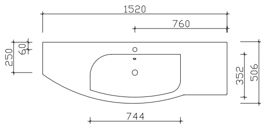
Width 1520 mm GWTR65-1510-L
