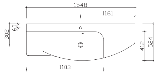
Width 1548 mm RD-MMWTR65-1548-R
